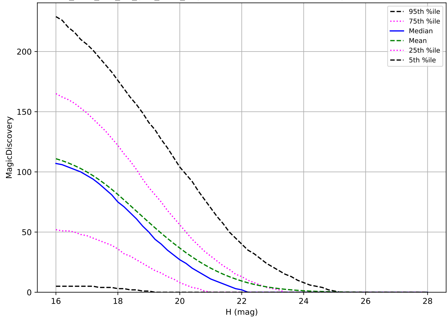
too_elab_r32_d2_griz_v3.4_10yrs: NEO 6 detections in 60 nights detection loss
