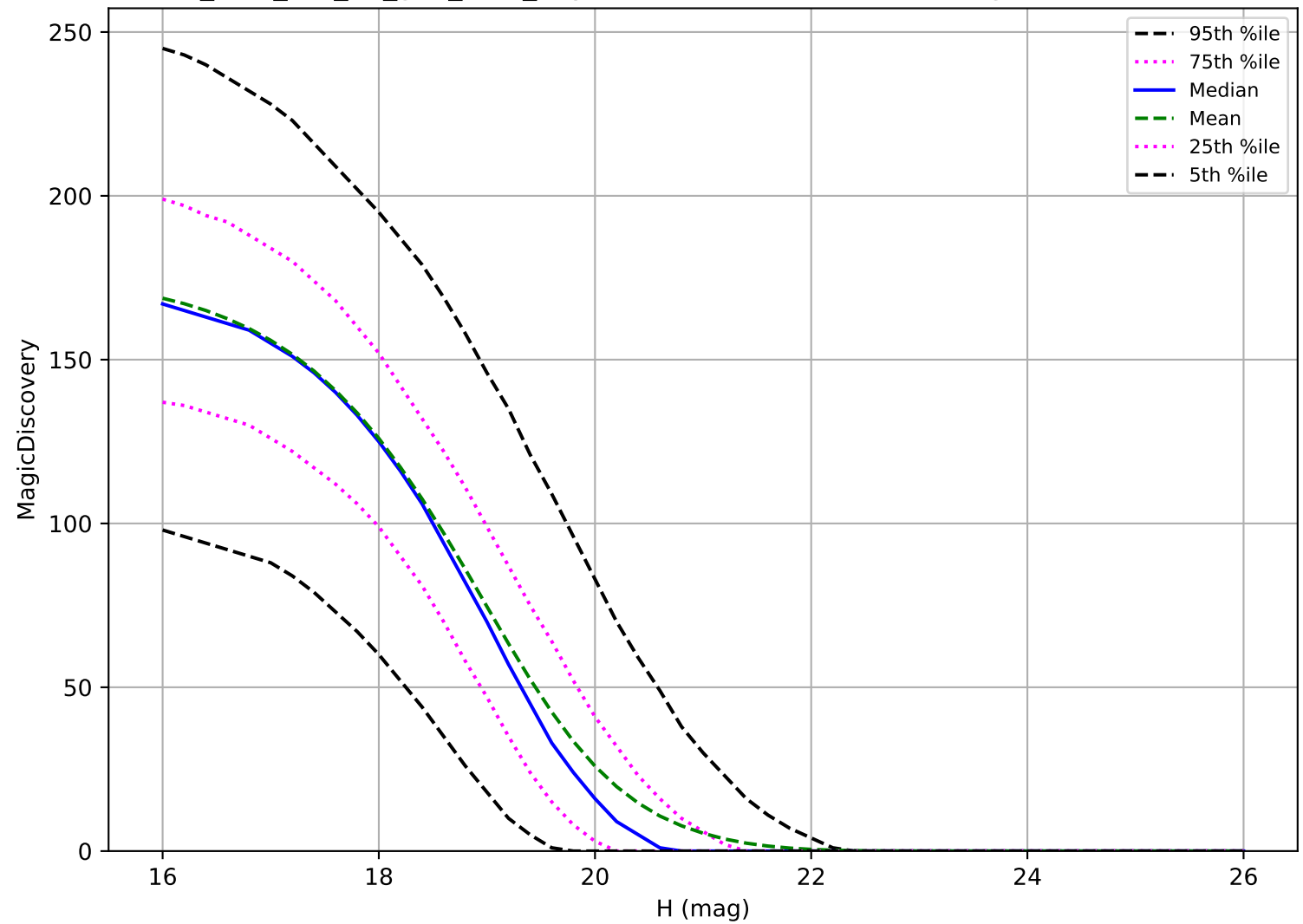
too_elab_r32_d2_griz_v3.4_10yrs: MBA 6 detections in 60 nights detection loss
