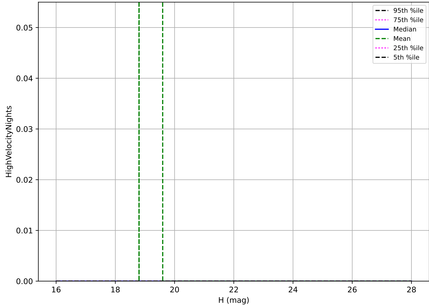
too_elab_r32_d2_griz_v3.4_10yrs: Vatira High velocity pair detection loss
