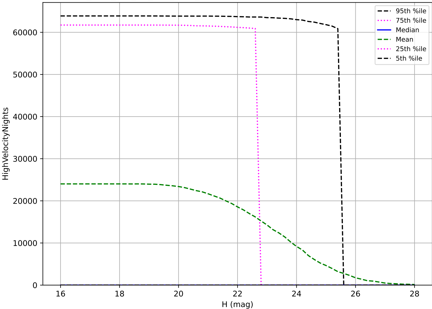
too_elab_r32_d2_griz_v3.4_10yrs: PHA High velocity pair detection loss
