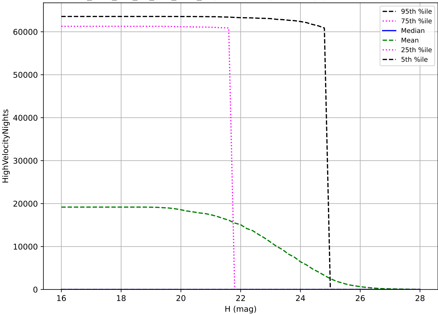
too_elab_r32_d2_griz_v3.4_10yrs: NEO High velocity pair detection loss
