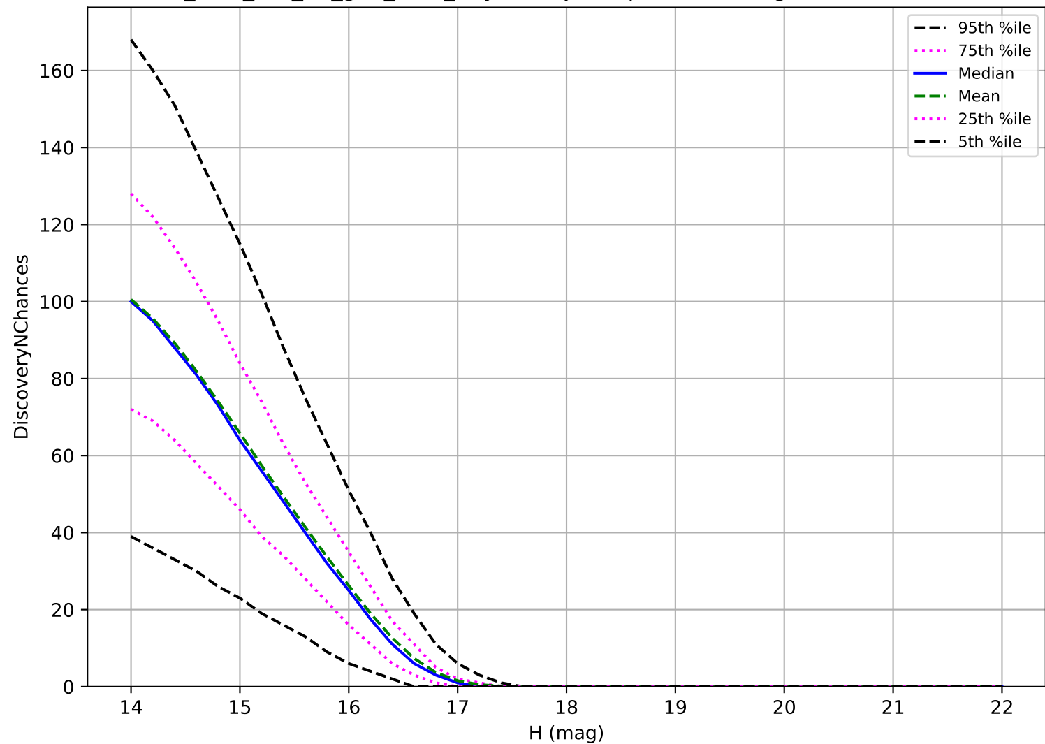
too_elab_r32_d2_griz_v3.4_10yrs: Trojan 3 pairs in 15 nights detection loss
