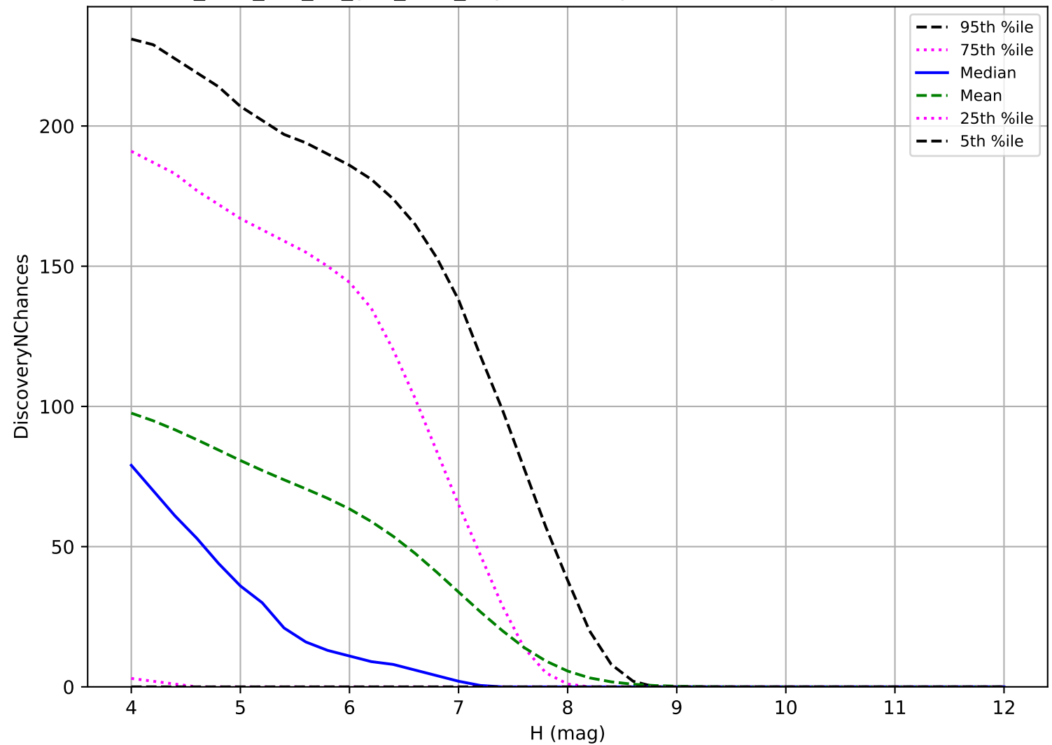
too_elab_r32_d2_griz_v3.4_10yrs: TNO 3 pairs in 15 nights detection loss
