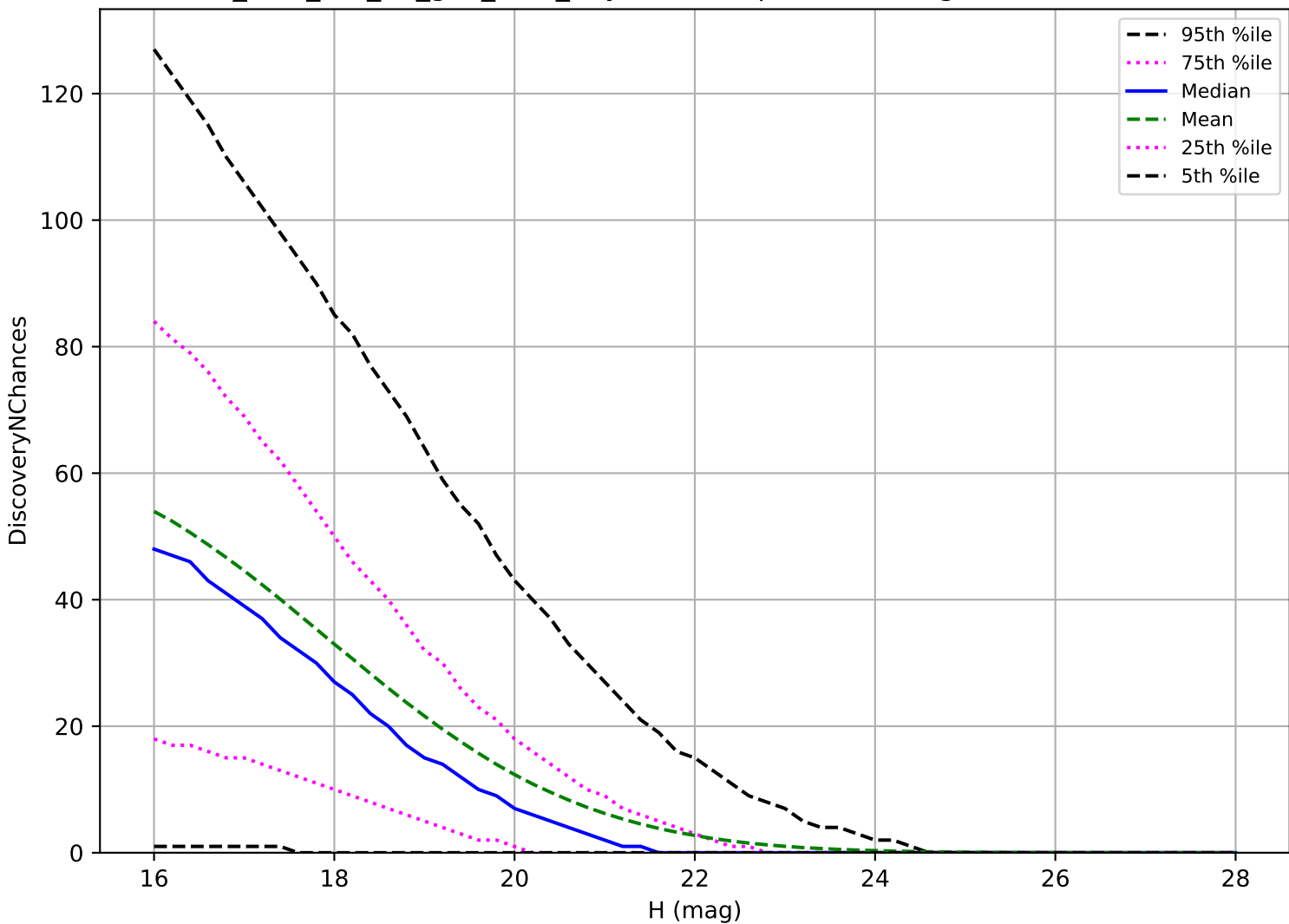
too_elab_r32_d2_griz_v3.4_10yrs: PHA 3 pairs in 15 nights detection loss
