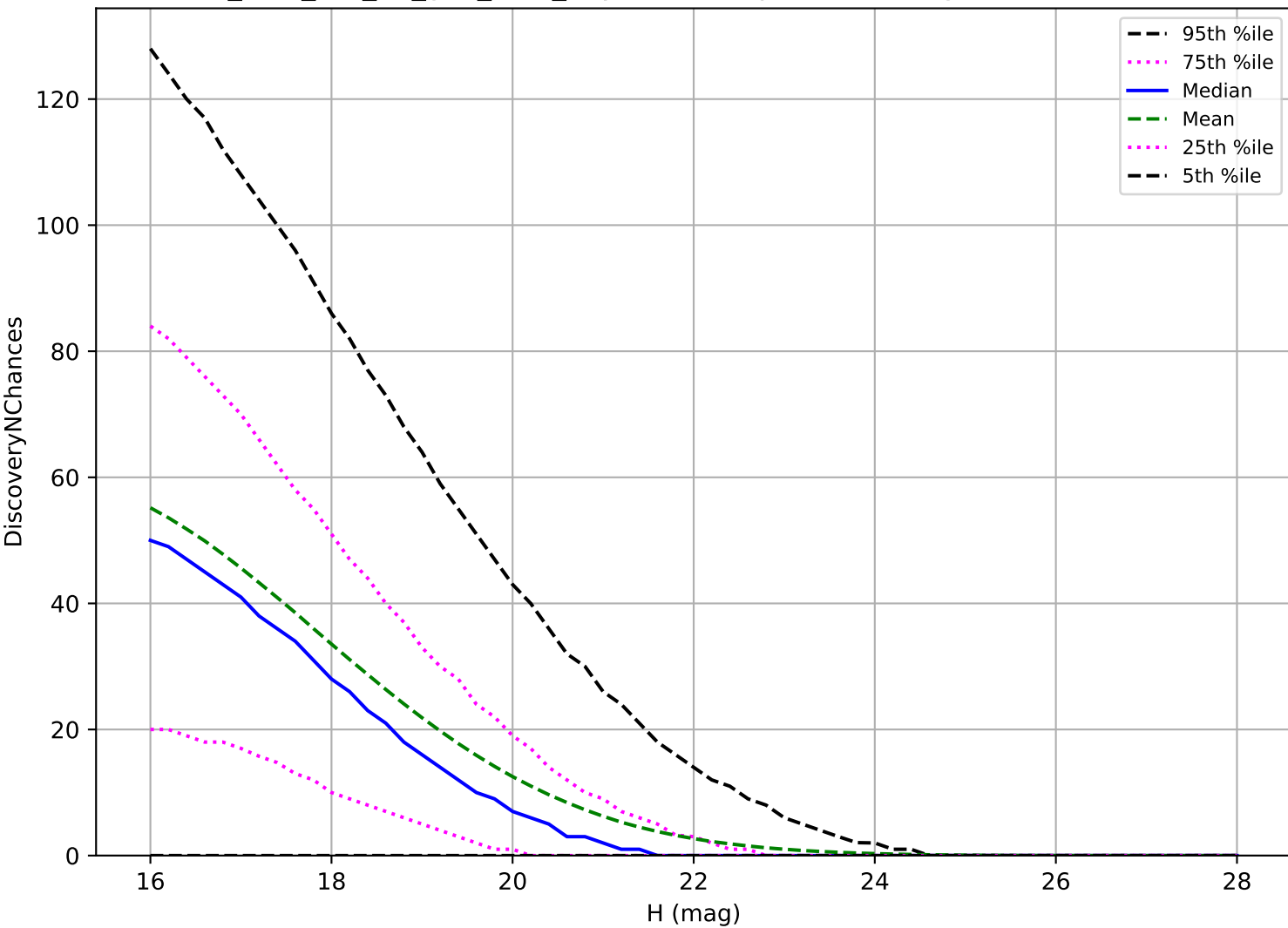
too_elab_r32_d2_griz_v3.4_10yrs: NEO 3 pairs in 15 nights detection loss
