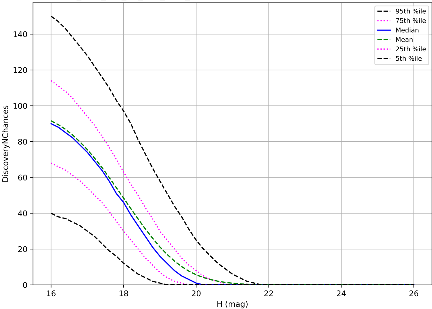
too_elab_r32_d2_griz_v3.4_10yrs: MBA 3 pairs in 15 nights detection loss
