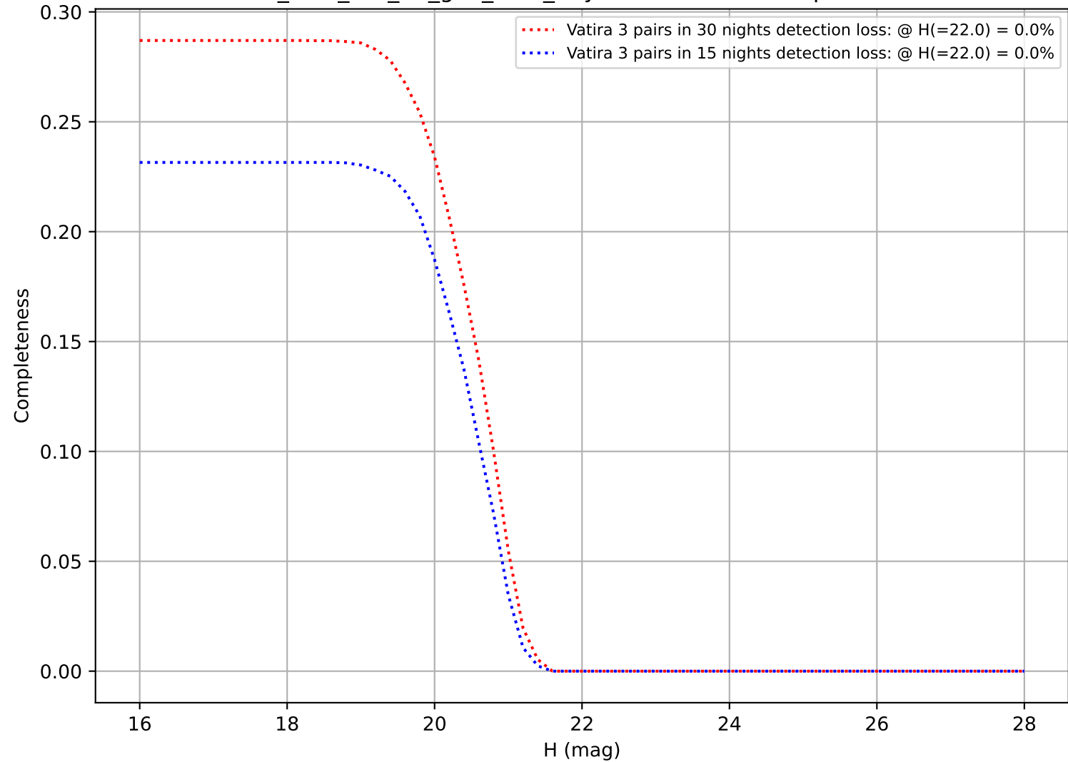
too_elab_r32_d2_griz_v3.4_10yrs: DifferentialCompleteness
