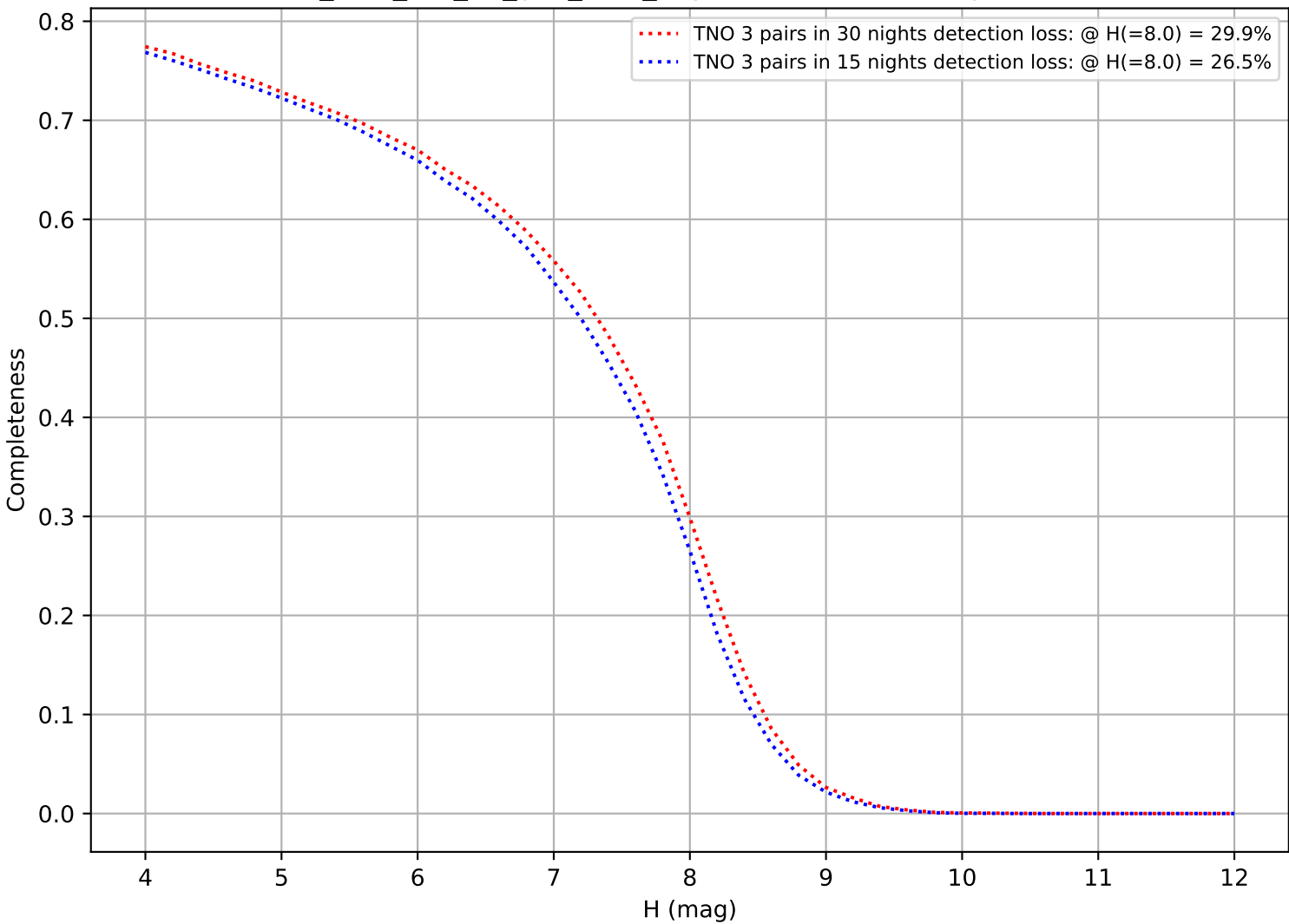
too_elab_r32_d2_griz_v3.4_10yrs: DifferentialCompleteness
