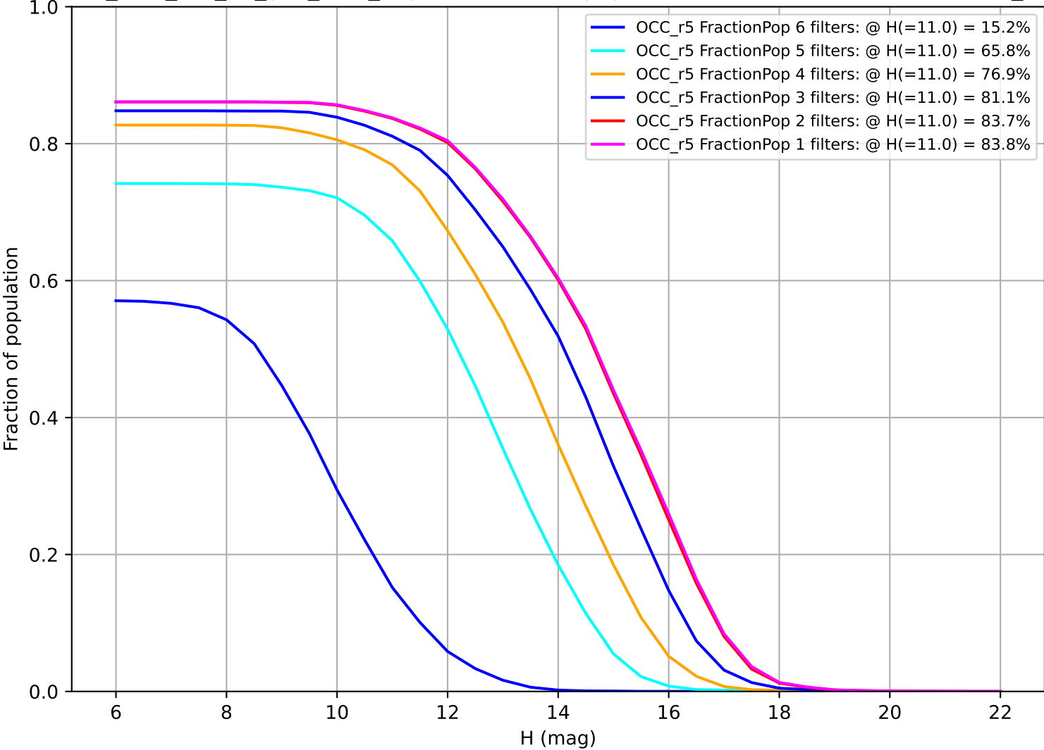
too_elab_r32_d2_griz_v3.4_10yrs: Fraction of population with colors in X filters OCC_r5
