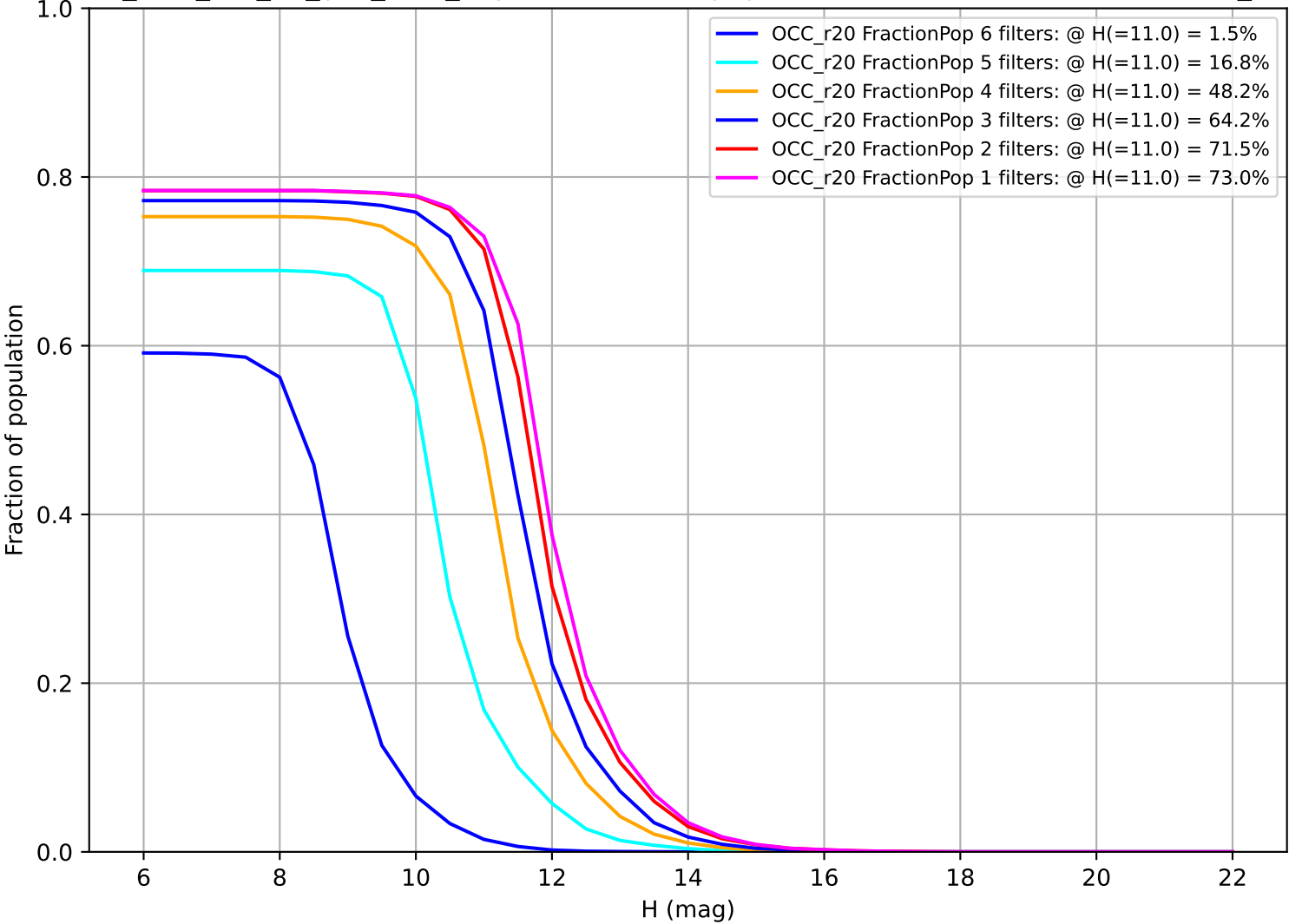
too_elab_r32_d2_griz_v3.4_10yrs: Fraction of population with colors in X filters OCC_r20
