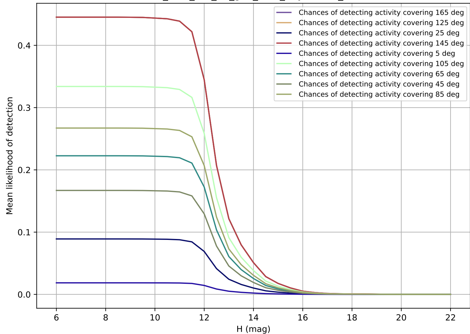
too_elab_r32_d2_griz_v3.4_10yrs OCC_r20
