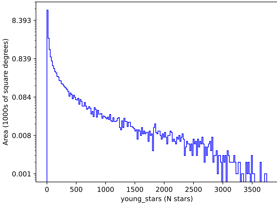
too_elab_r32_d2_griz_v3.4_10yrs : young_stars
