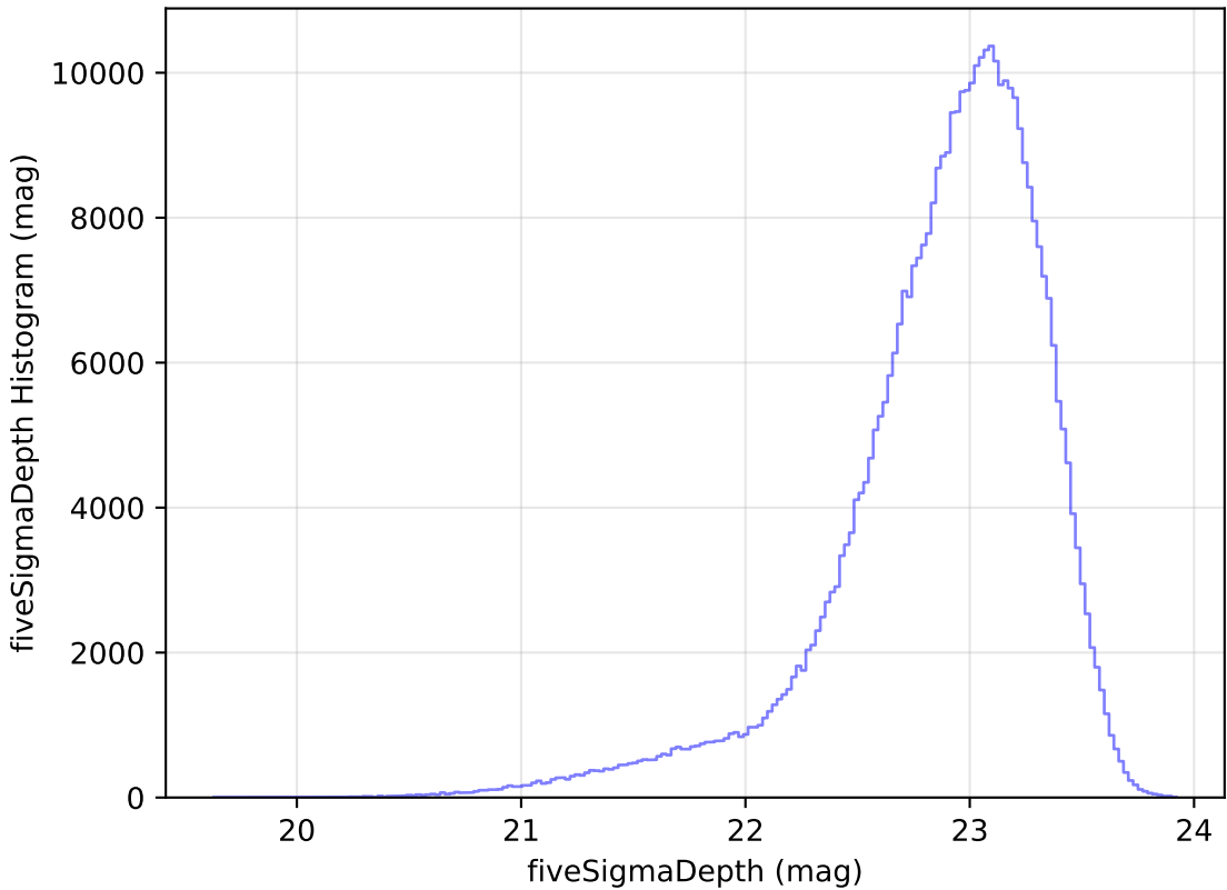
too_elab_r32_d2_griz_v3.4_10yrs z: fiveSigmaDepth Histogram
