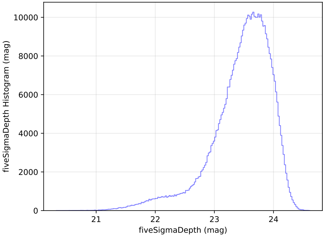
too_elab_r32_d2_griz_v3.4_10yrs i: fiveSigmaDepth Histogram
