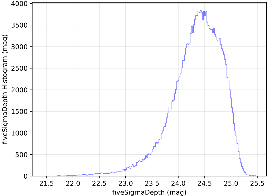
too_elab_r32_d2_griz_v3.4_10yrs g: fiveSigmaDepth Histogram
