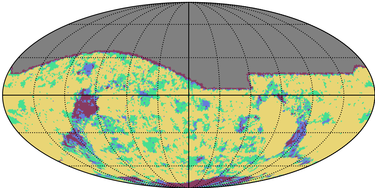
too_elab_r32_d2_griz_v3.4_10yrs g band: YearCoverage night
