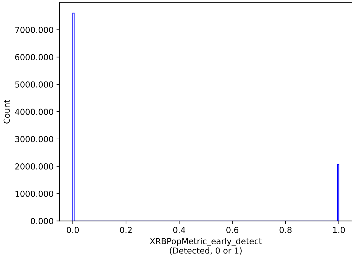
too_elab_r32_d2_griz_v3.4_10yrs : XRBPpopMetric_early_detect
