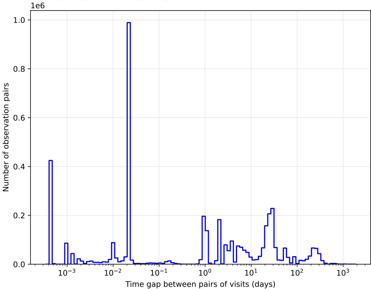
too_elab_r32_d2_griz_v3.4_10yrs y band: Tgaps observationStartMJD
