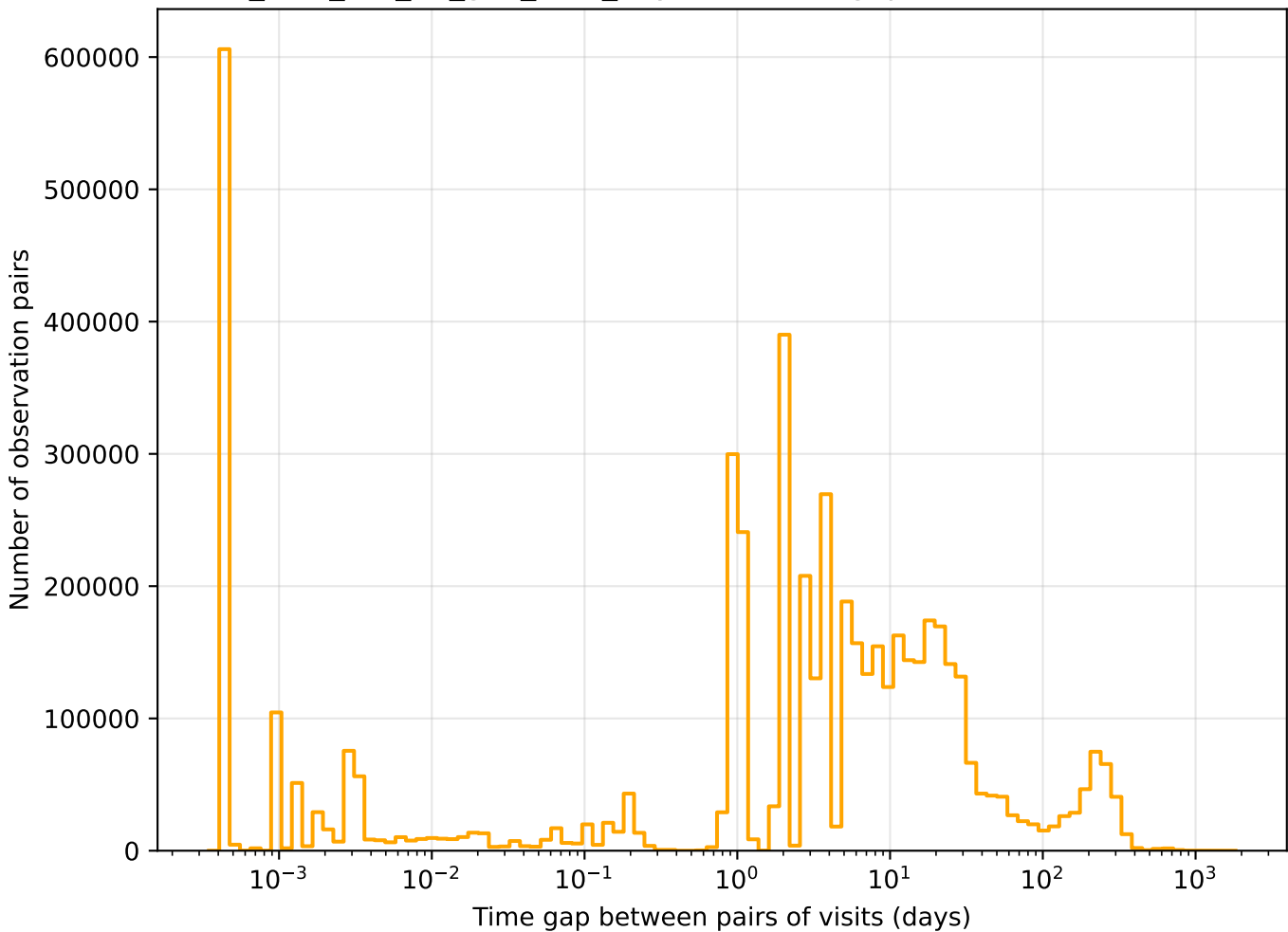
too_elab_r32_d2_griz_v3.4_10yrs r band: Tgaps observationStartMJD
