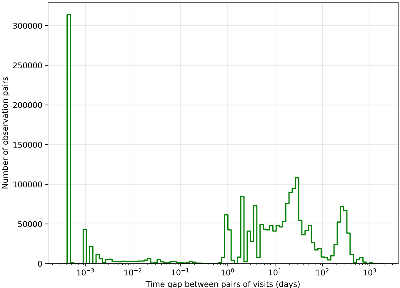
too_elab_r32_d2_griz_v3.4_10yrs g band: Tgaps observationStartMJD
