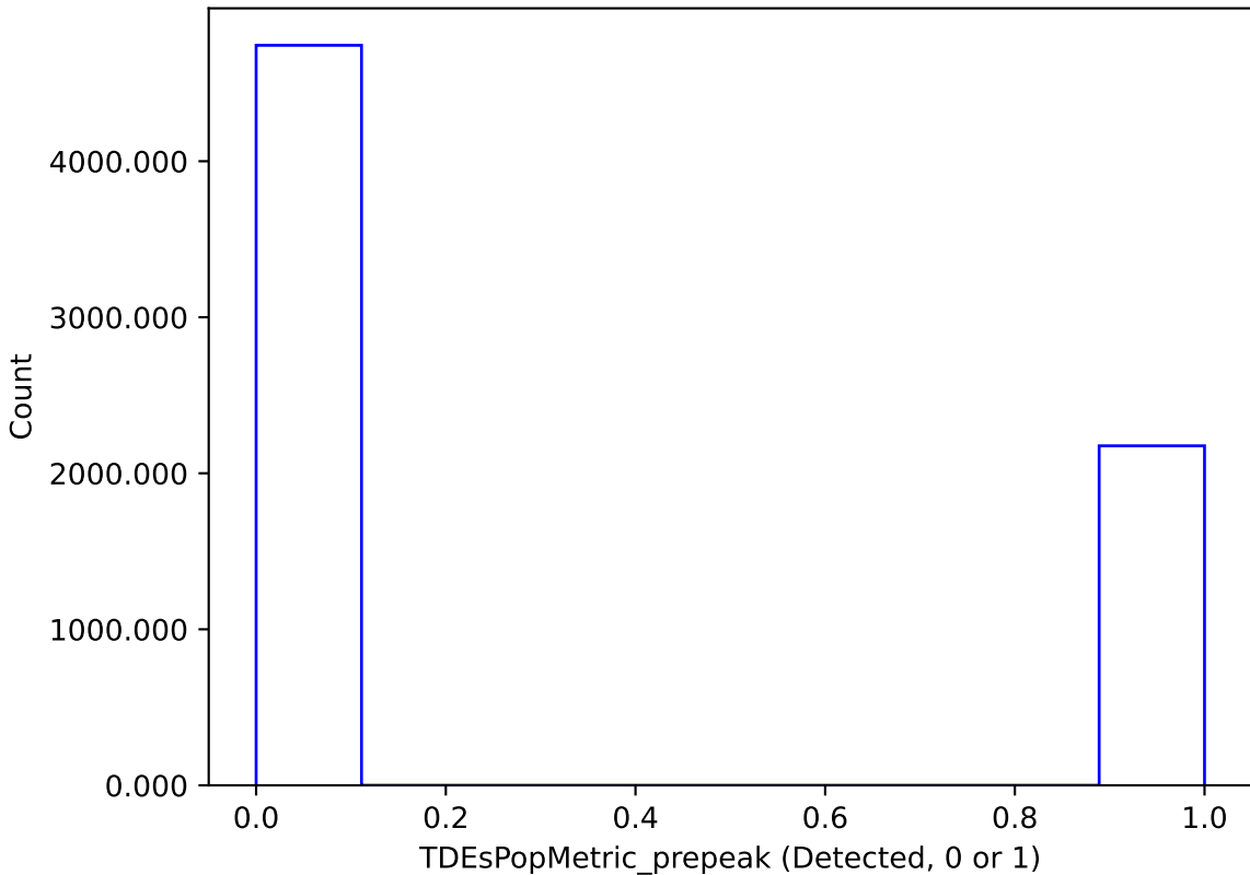
too_elab_r32_d2_griz_v3.4_10yrs : TDEsPopMetric_prepeak
