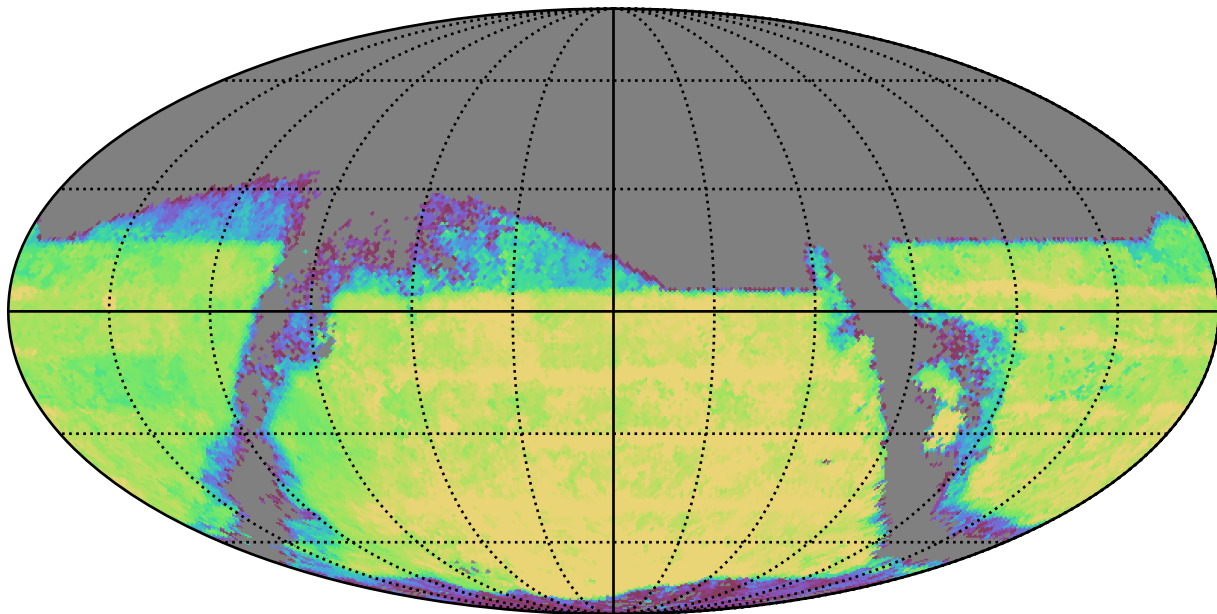
too_elab_r32_d2_griz_v3.4_10yrs : TDC_season
