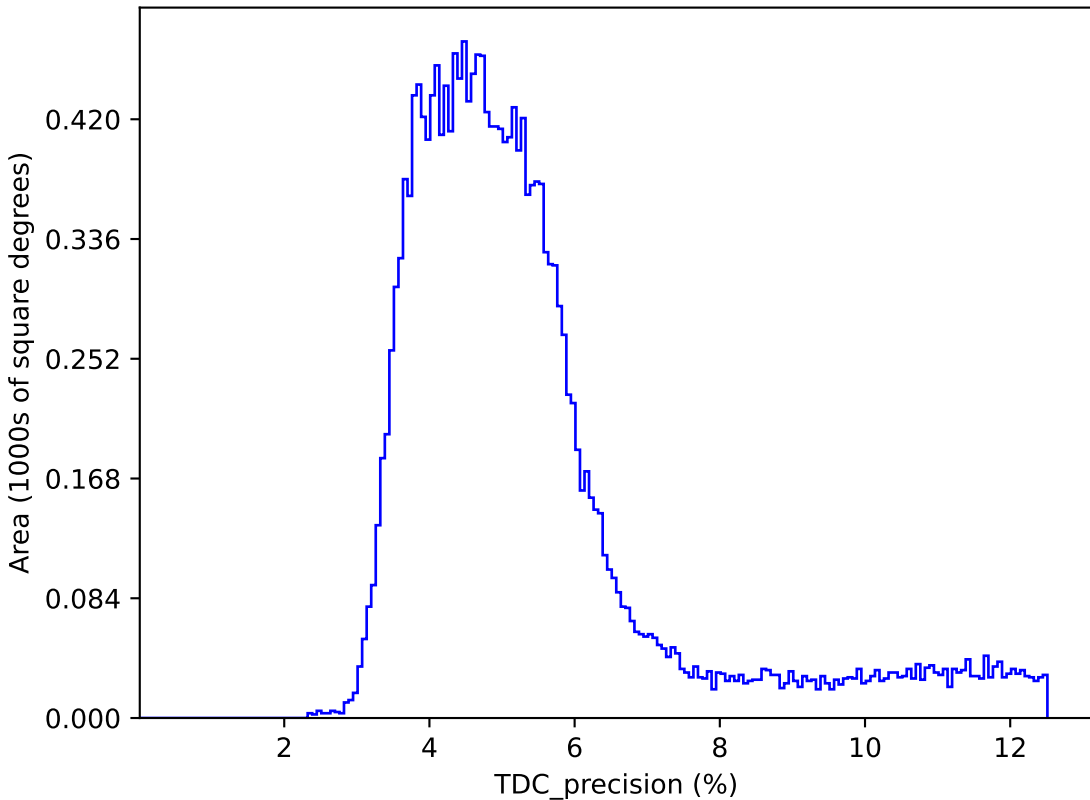
too_elab_r32_d2_griz_v3.4_10yrs : TDC_precision
