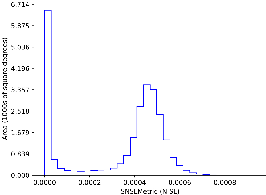
too_elab_r32_d2_griz_v3.4_10yrs : SNSLMetric
