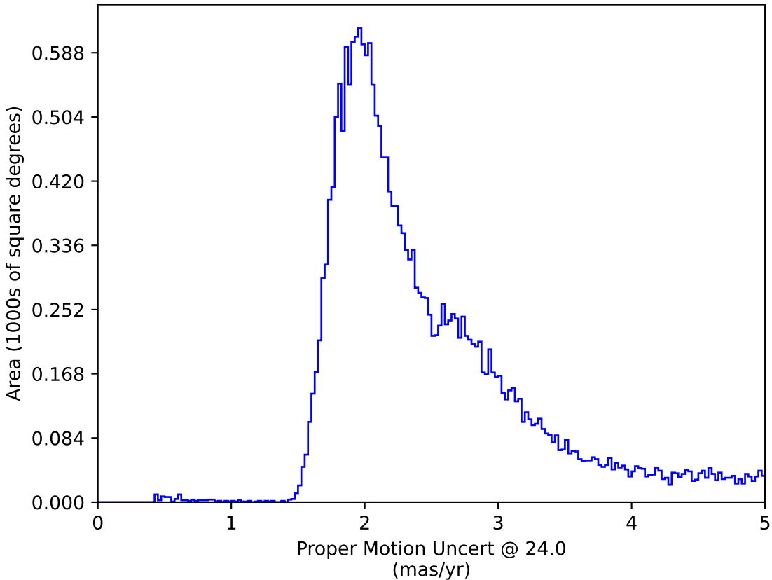
too_elab_r32_d2_griz_v3.4_10yrs : Proper Motion Uncert @ 24.0
