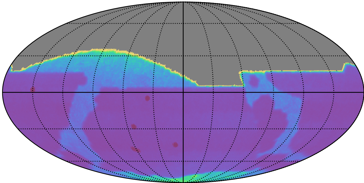
too_elab_r32_d2_griz_v3.4_10yrs : Proper Motion Uncert @ 20.5
