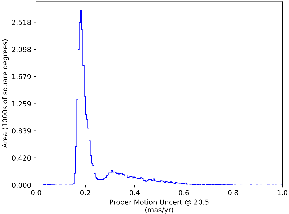
too_elab_r32_d2_griz_v3.4_10yrs : Proper Motion Uncert @ 20.5
