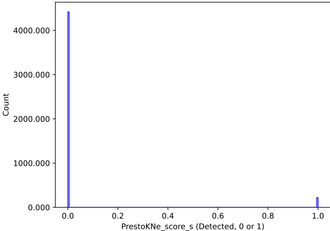
too_elab_r32_d2_griz_v3.4_10yrs : PrestoKNe_score_s
