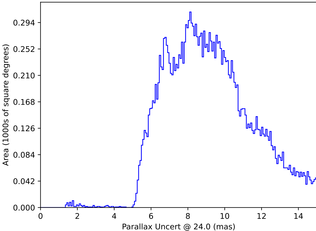
too_elab_r32_d2_griz_v3.4_10yrs : Parallax Uncert @ 24.0
