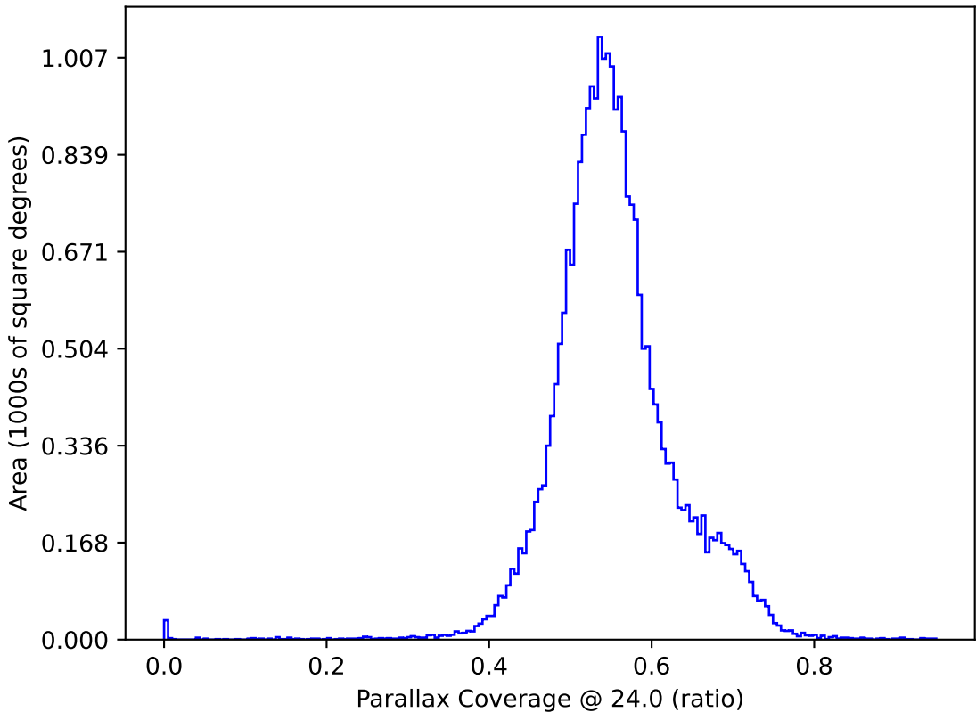
too_elab_r32_d2_griz_v3.4_10yrs : Parallax Coverage @ 24.0
