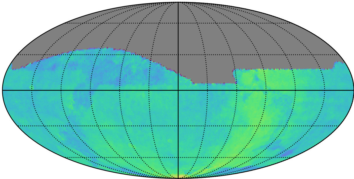
too_elab_r32_d2_griz_v3.4_10yrs : Parallax Coverage @ 22.4
