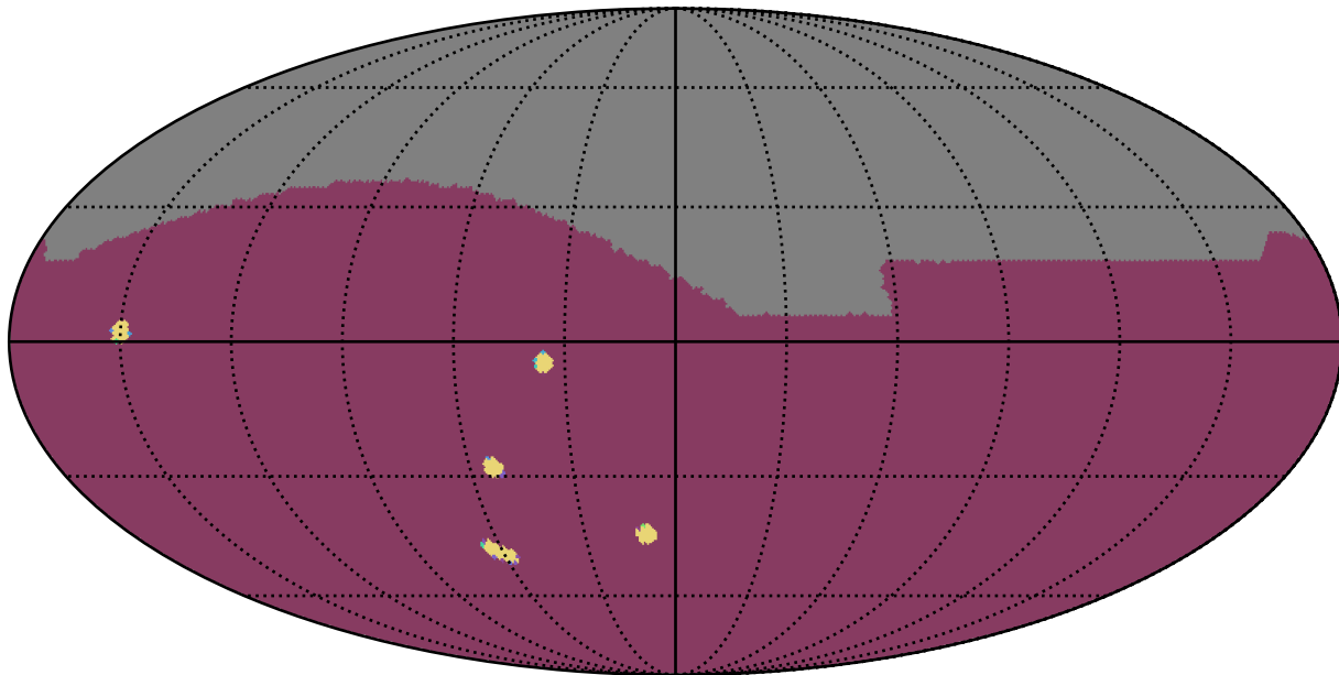
too_elab_r32_d2_griz_v3.4_10yrs : NumberOfQuickRevisits
