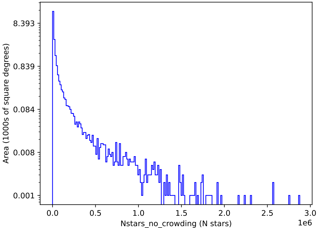
too_elab_r32_d2_griz_v3.4_10yrs u: Nstars_no_crowding
