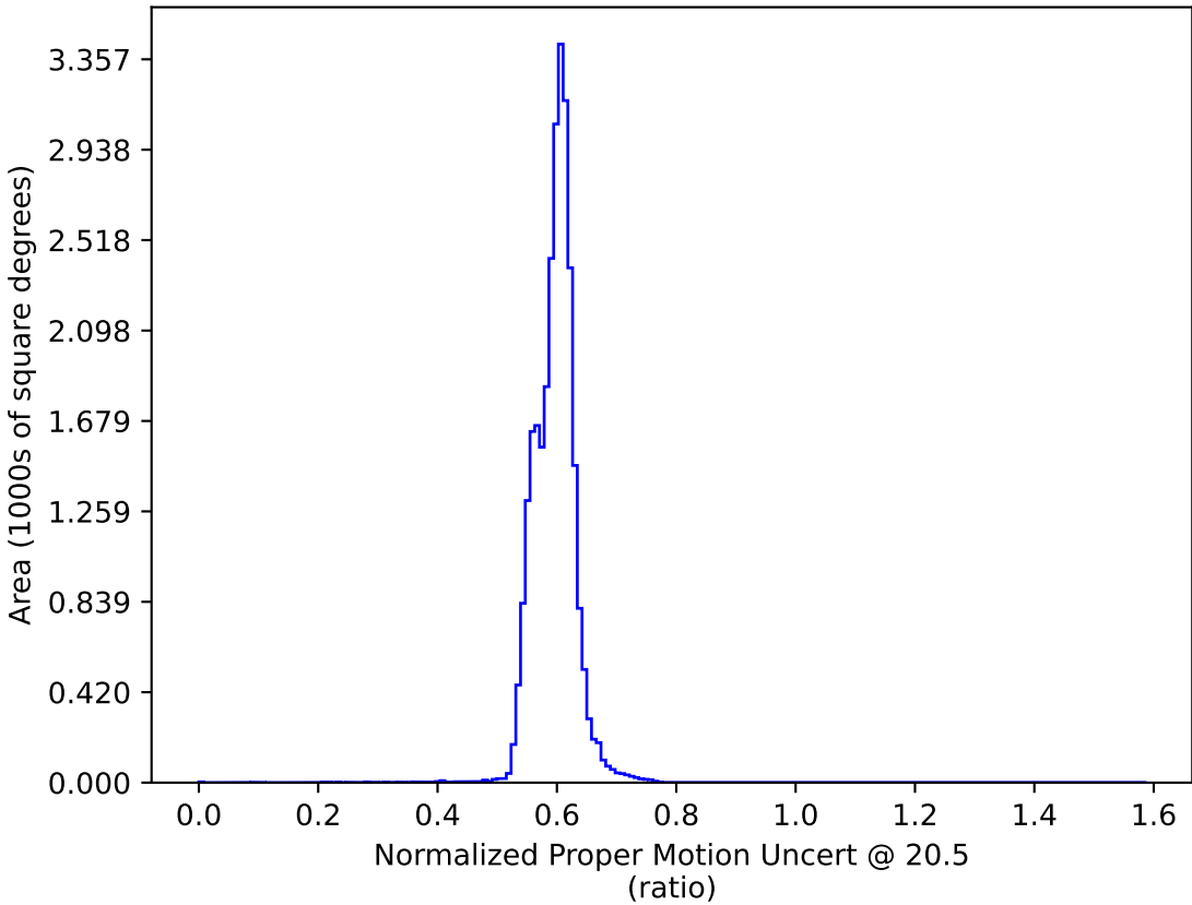
too_elab_r32_d2_griz_v3.4_10yrs : Normalized Proper Motion Uncert @ 20.5
