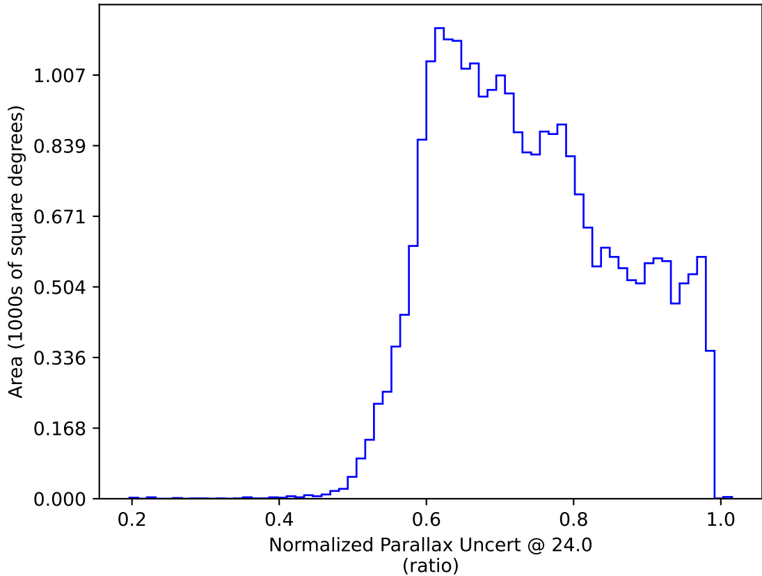
too_elab_r32_d2_griz_v3.4_10yrs : Normalized Parallax Uncert @ 24.0
