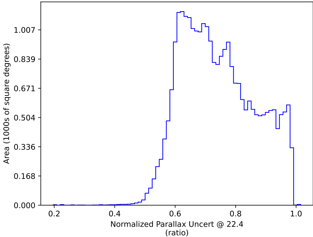
too_elab_r32_d2_griz_v3.4_10yrs : Normalized Parallax Uncert @ 22.4
