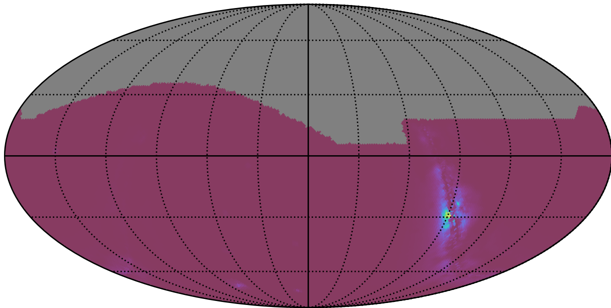
too_elab_r32_d2_griz_v3.4_10yrs : NlcPoints
