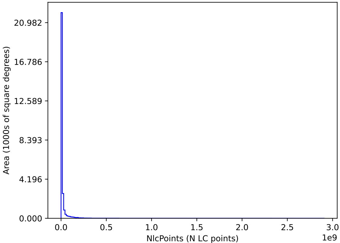
too_elab_r32_d2_griz_v3.4_10yrs : NlcPoints
