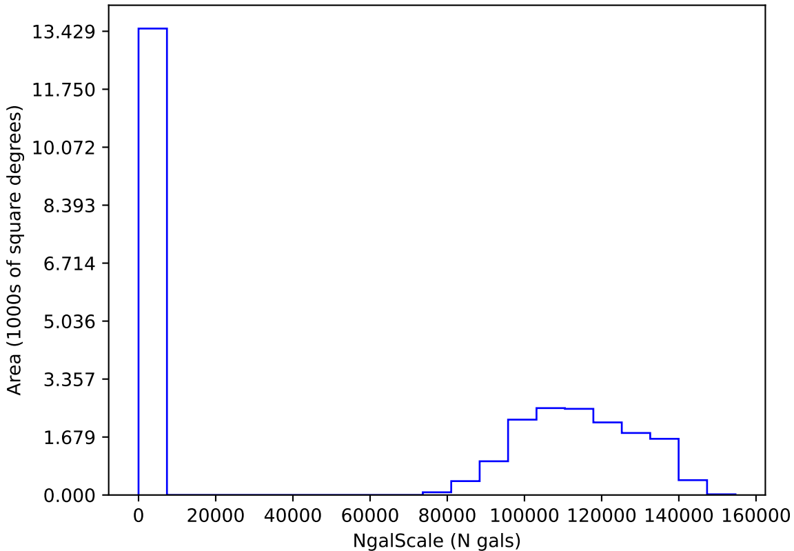
too_elab_r32_d2_griz_v3.4_10yrs i: NgalScale
