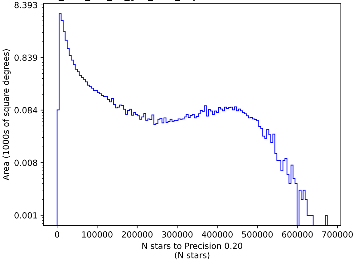
too_elab_r32_d2_griz_v3.4_10yrs i: N stars to Precision 0.20
