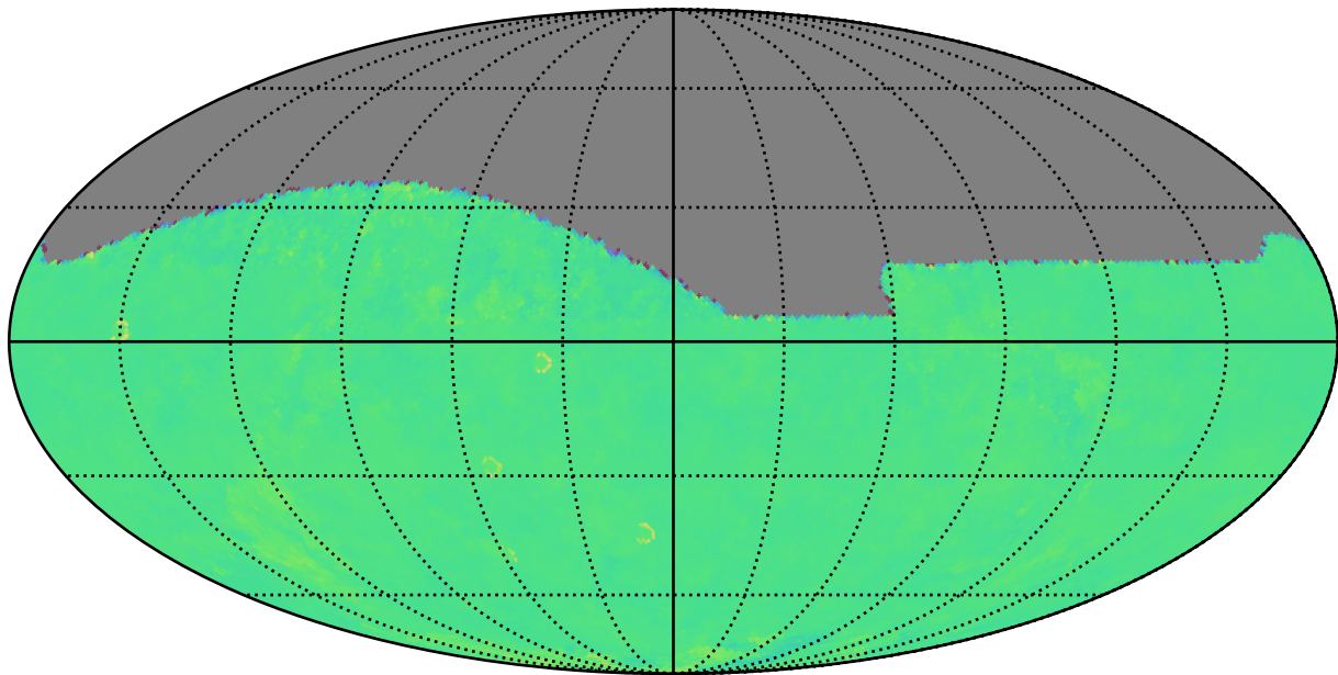
too_elab_r32_d2_griz_v3.4_10yrs z: Kuiper rotTelPos
