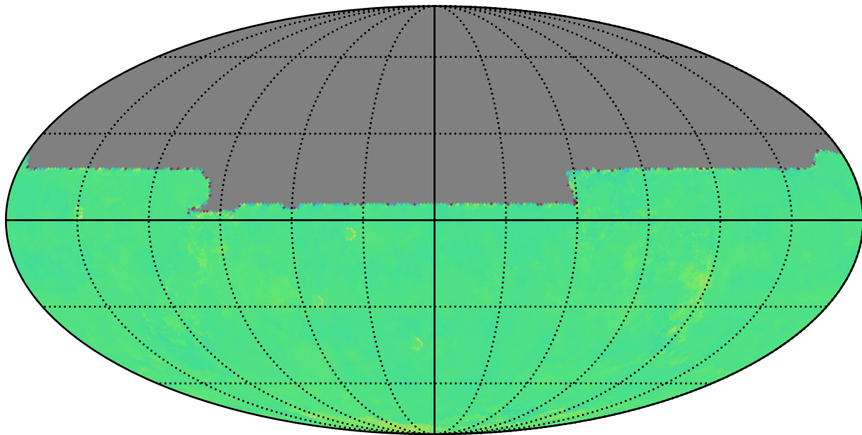
too_elab_r32_d2_griz_v3.4_10yrs y: Kuiper rotTelPos
