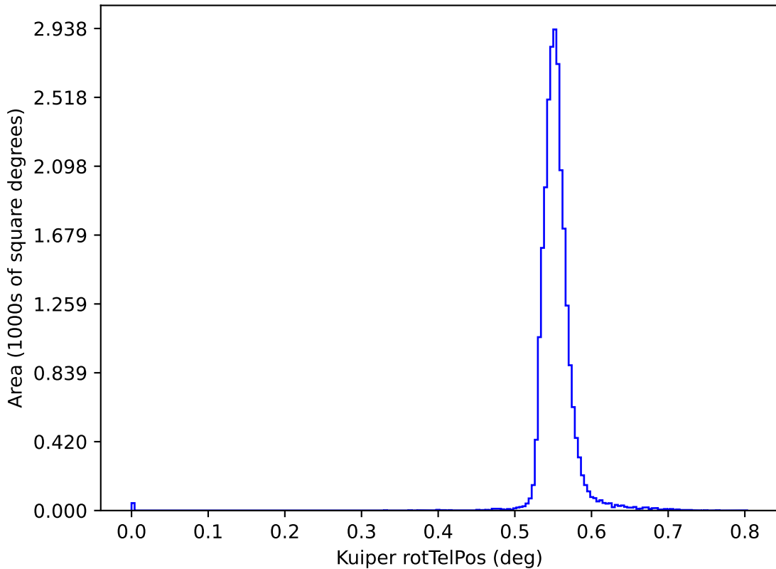
too_elab_r32_d2_griz_v3.4_10yrs y: Kuiper rotTelPos
