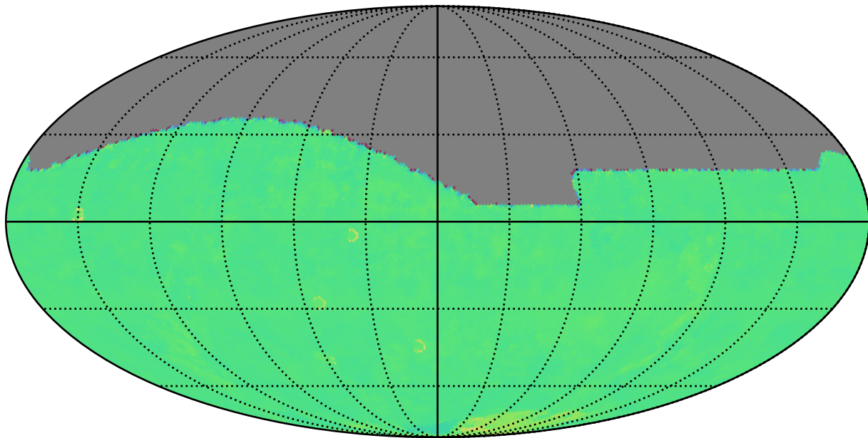
too_elab_r32_d2_griz_v3.4_10yrs r: Kuiper rotTelPos
