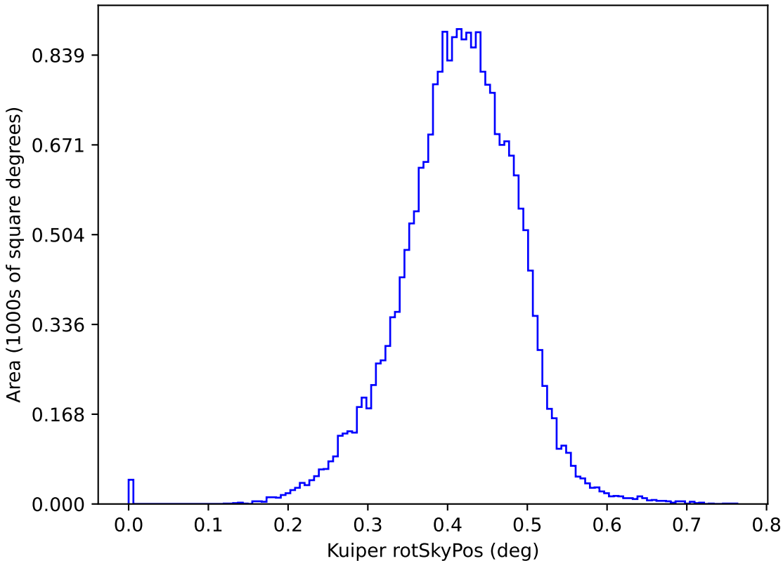
too_elab_r32_d2_griz_v3.4_10yrs y: Kuiper rotSkyPos
