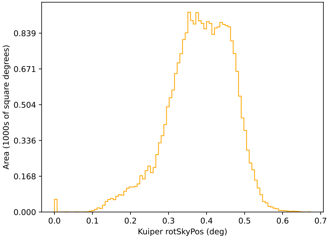
too_elab_r32_d2_griz_v3.4_10yrs r: Kuiper rotSkyPos
